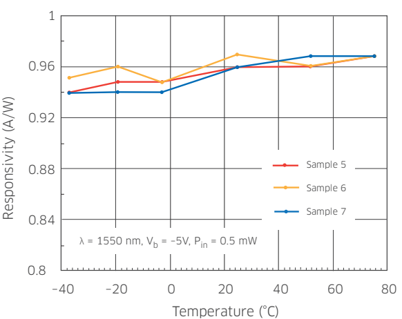
Responsivity vs. Temperature (EPM 605)
