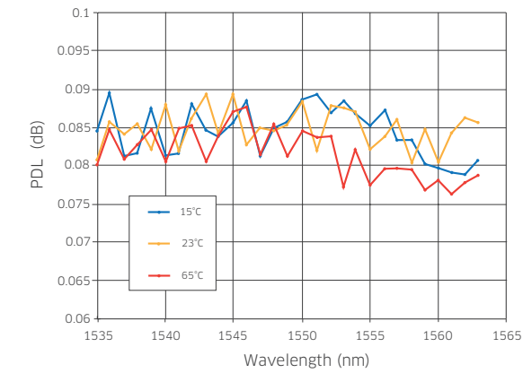
PDL vs. Wavelength, Temperature (EPM 605)
